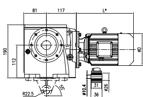
Torque arm-mounted with accessory (T) Weight: 17kg (Without motor and oil)
