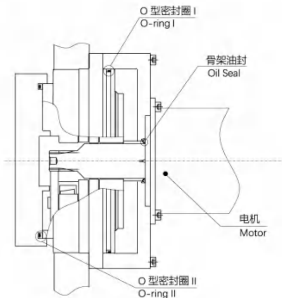
BXJ-80E及以下型号密封示意图 The seal diagram of BXJ-80E and the smaller
