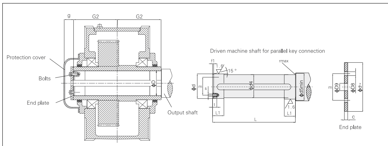
Type H2...H, H3...H, H4...H, B3...H, B4...H (Size 04–12)
