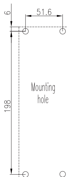
M1(0.75KW~5.5KW)'s dimensions, the unit is mm
