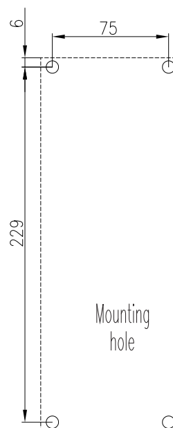
M2(5.5KW)'s dimensions, the unit is mm
